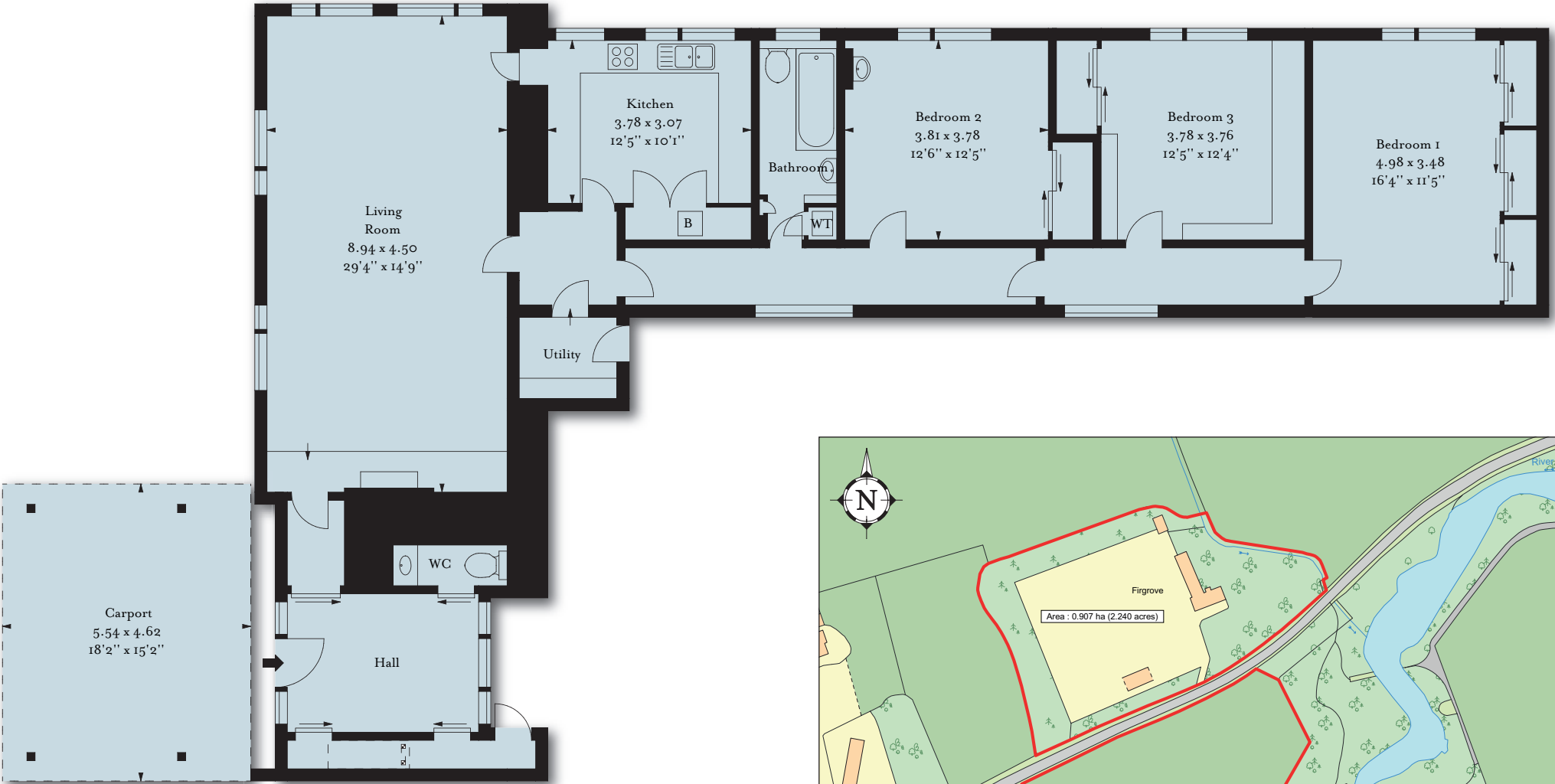
GROUND FLOOR
