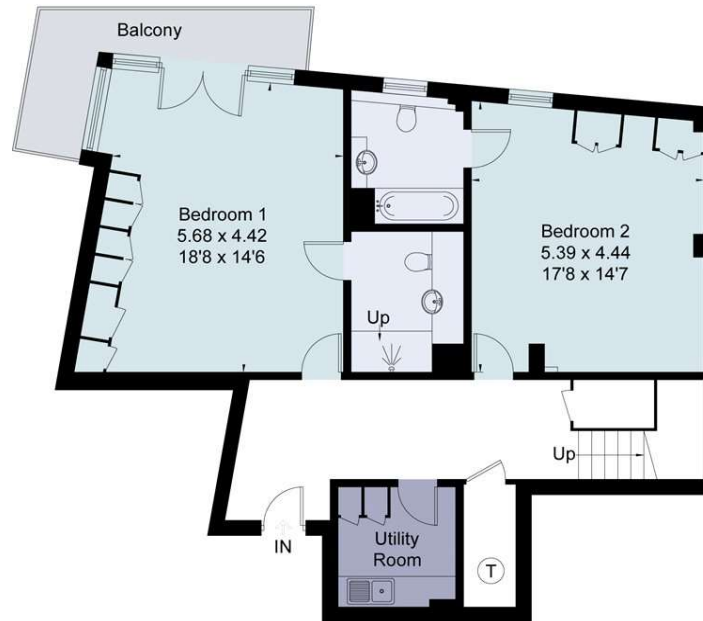
Fifth Floor
