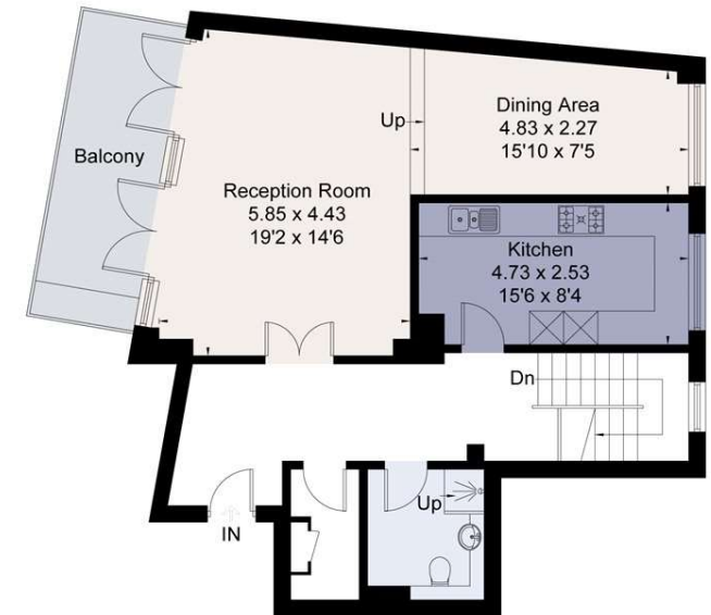
Sixth Floor
