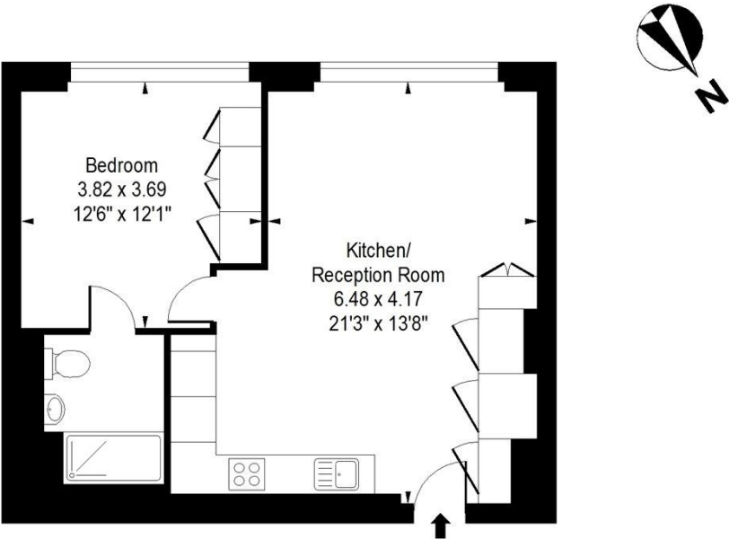
Fourth Floor
