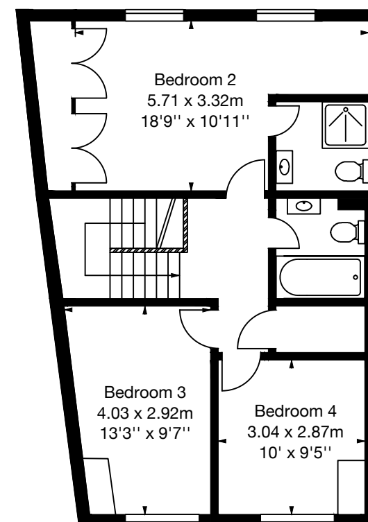
Second Floor
