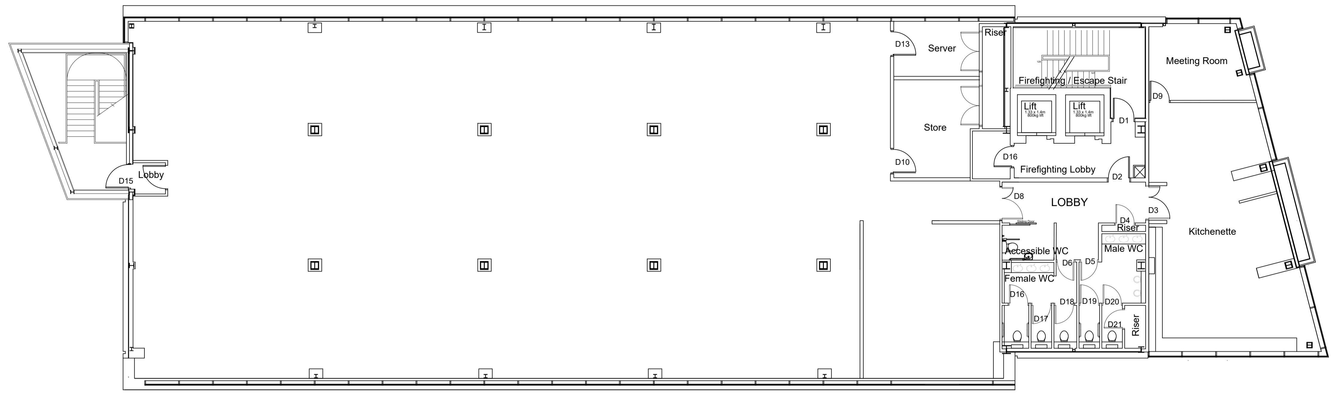
EXISTING THIRD FLOOR PLAN
