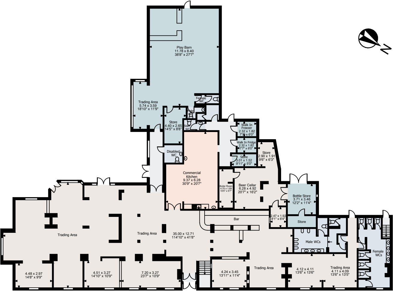
Ground Floor
