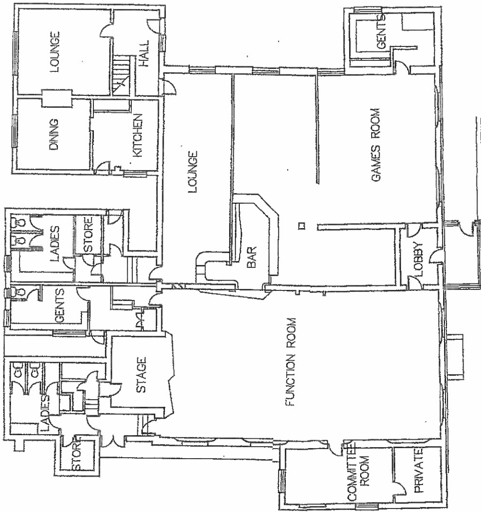
EXISTING PLAN 1:100
