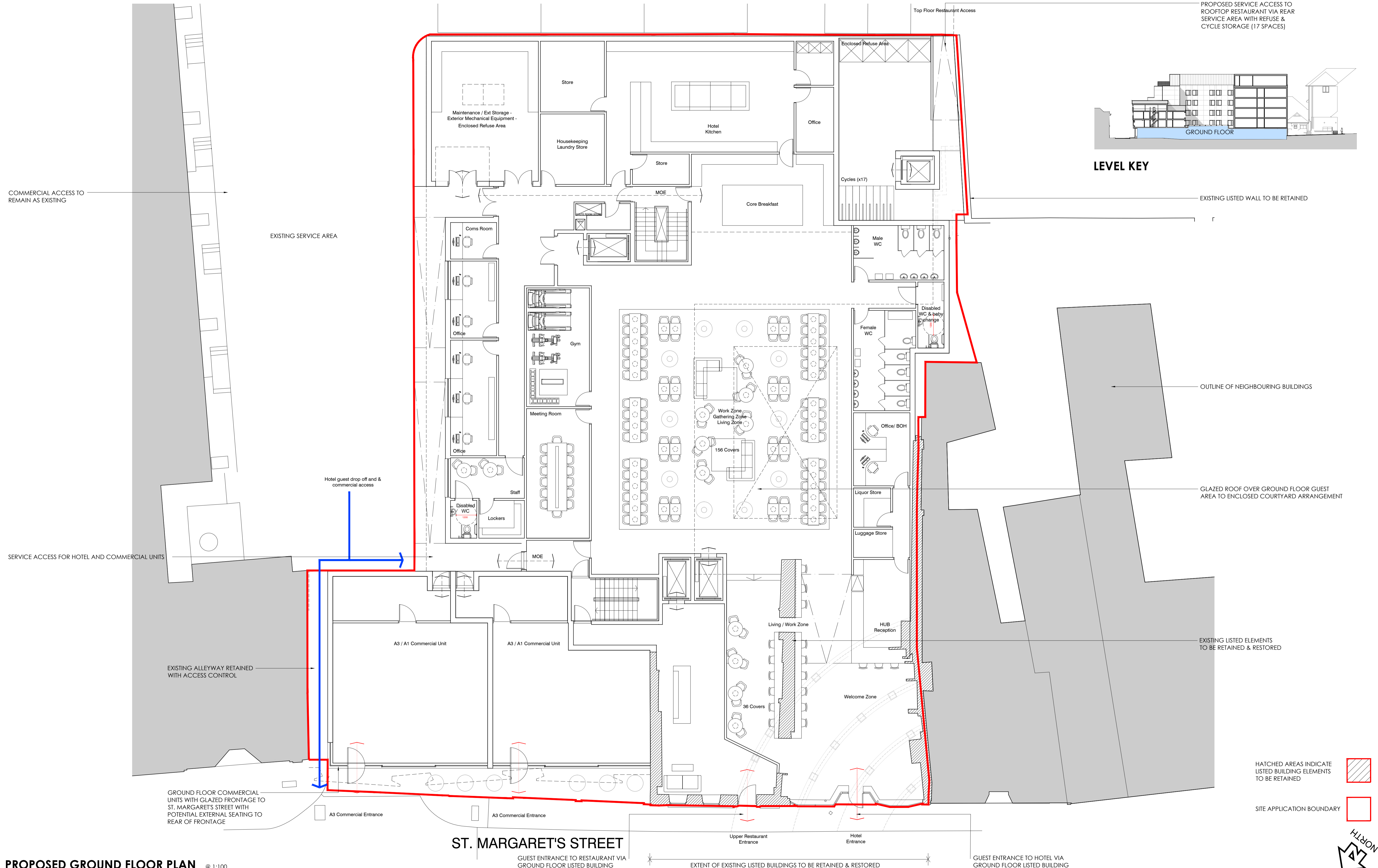
PROPOSED GROUND FLOOR PLAN @ 1:100
