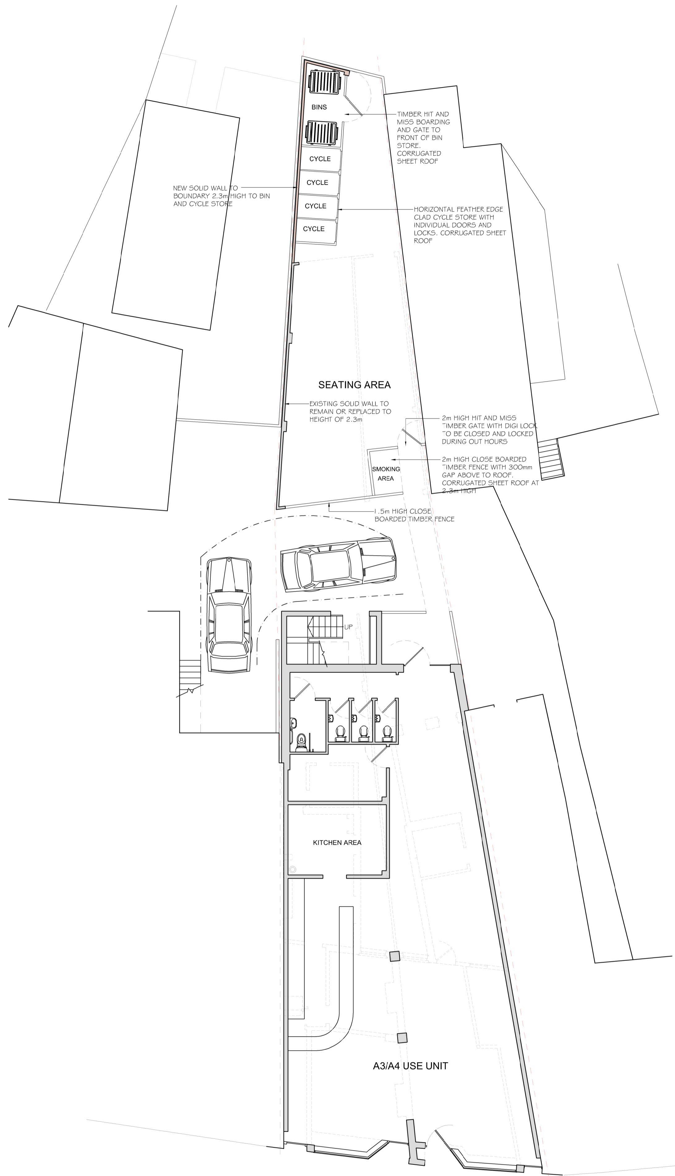
GROUND FLOOR 1:100
