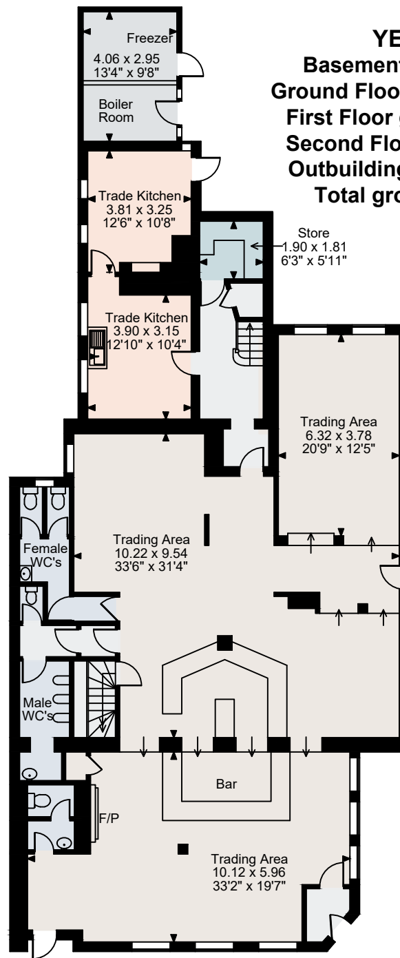
Ground Floor
