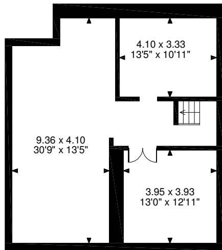
Cellar
