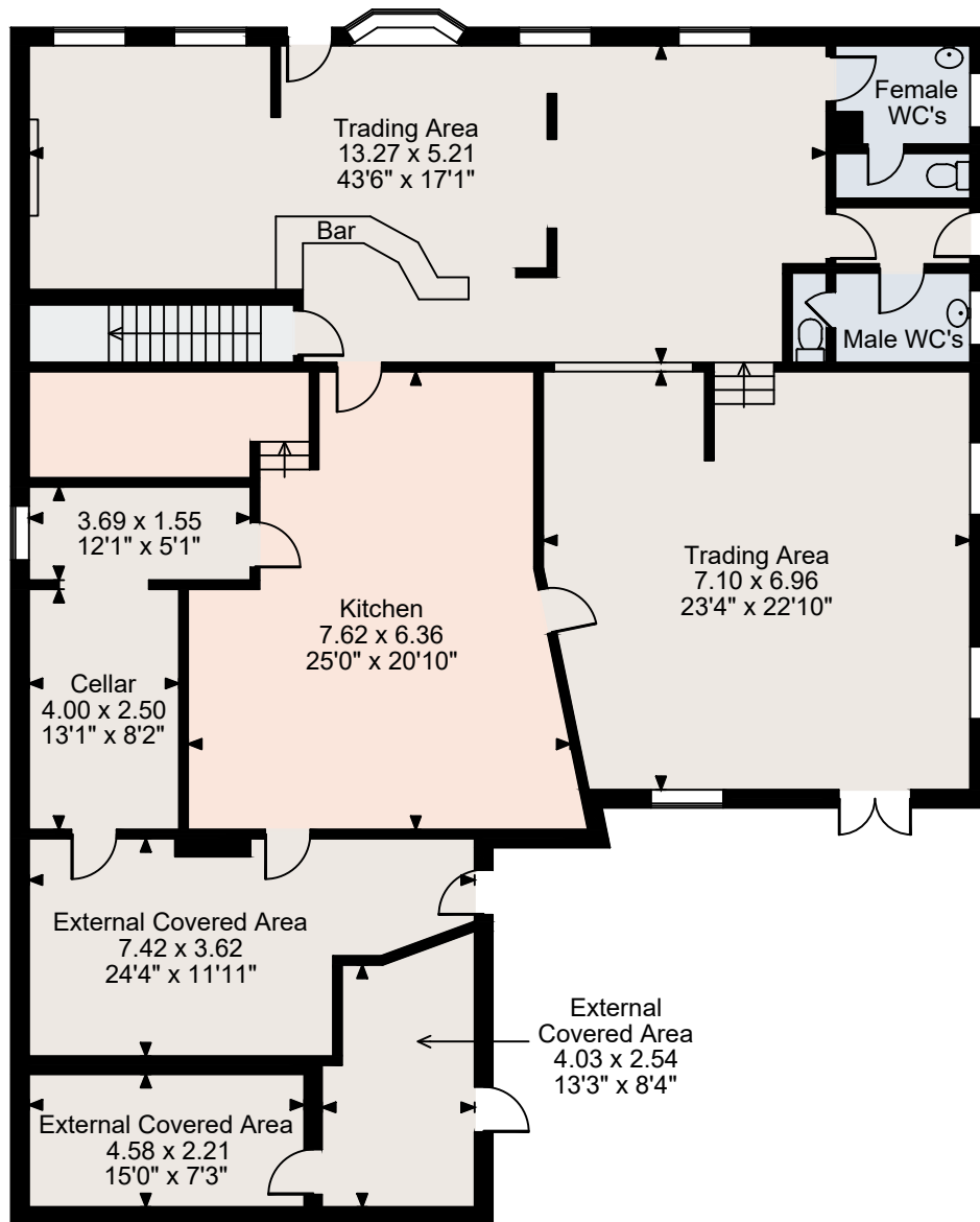
Ground Floor
