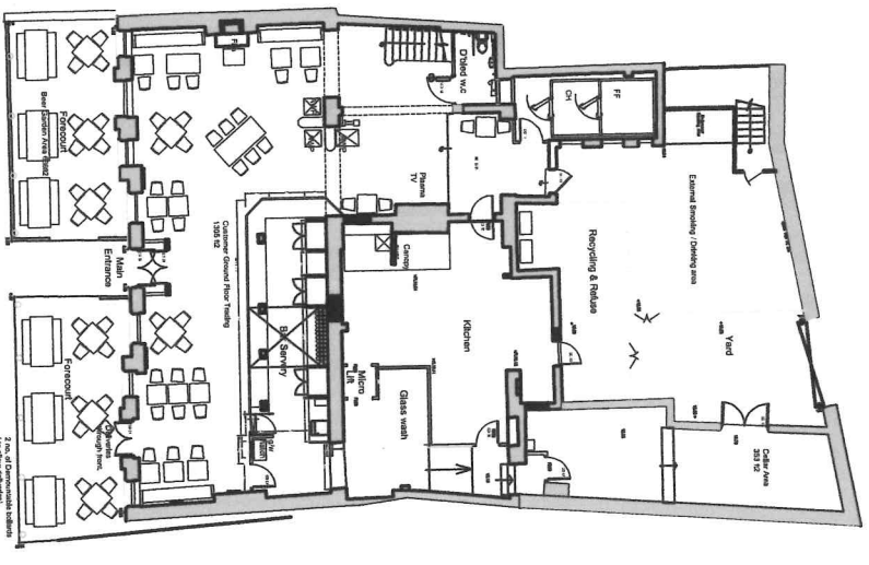
PROPOSED GROUND FLOOR PLAN High Street
