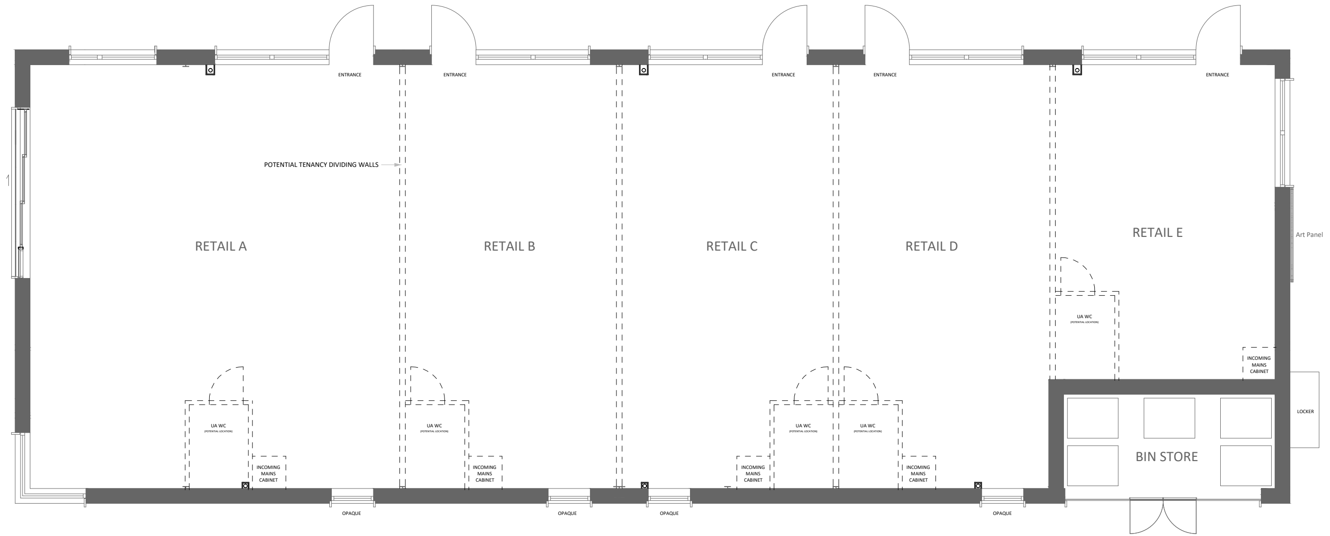
1 Planning 1.0 Ground Floor 1:50
