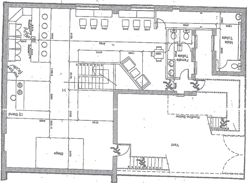
EXISTING FIRST FLOOR LAYOUT (VOODOO ROOM) SCALE: 1:100
