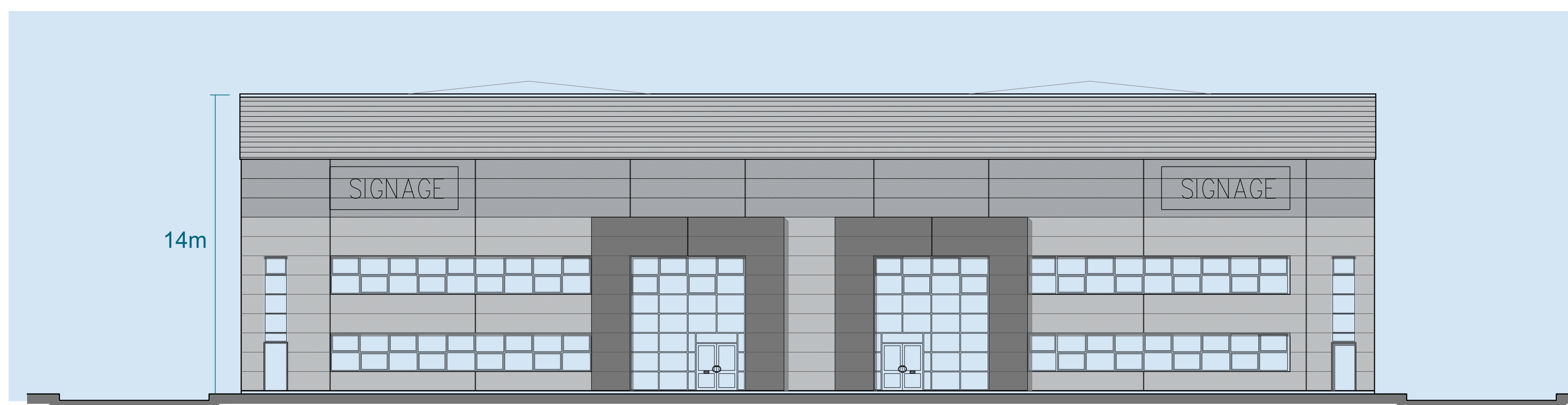
South Elevation
