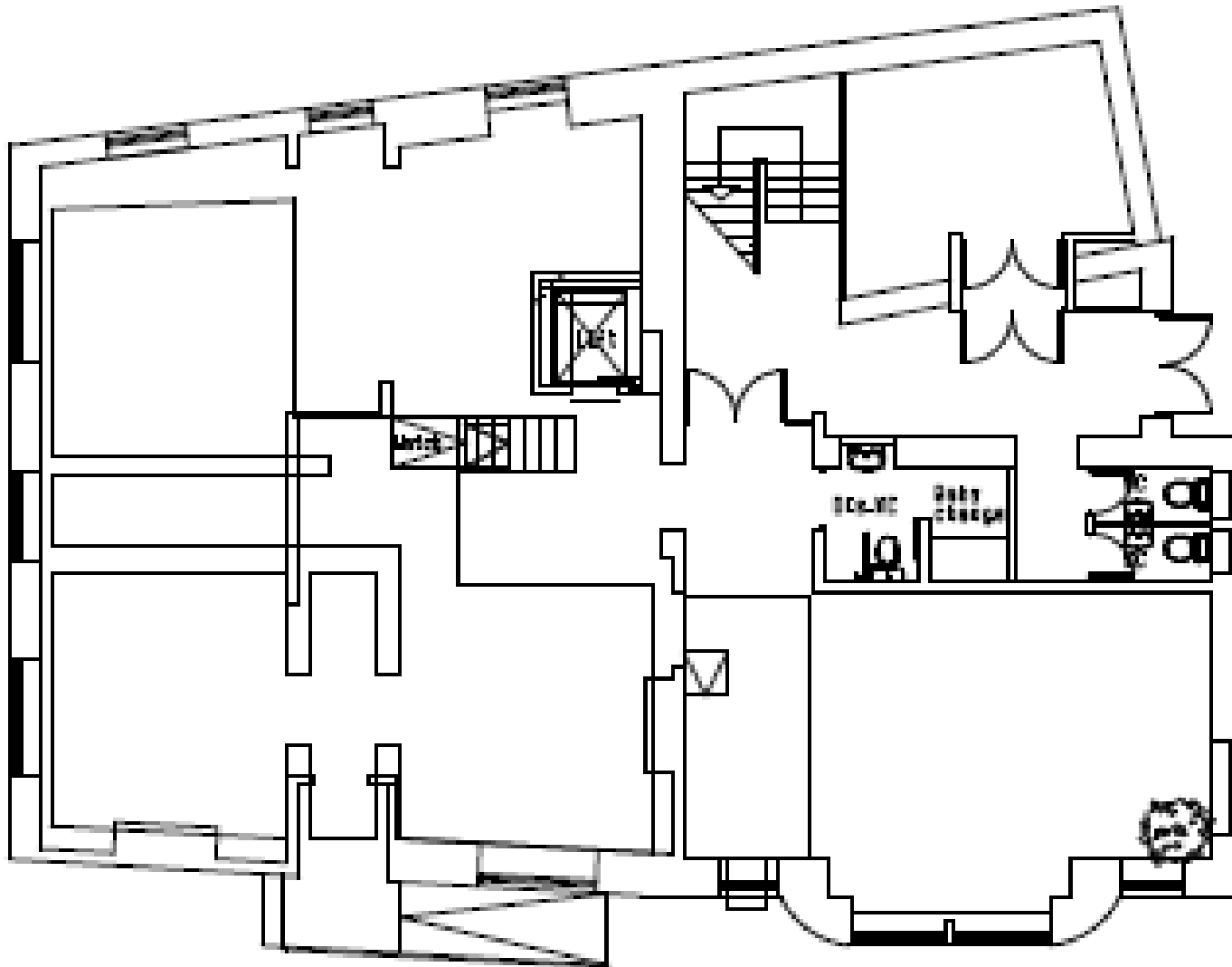
EXISTING CELLAR LAYOUT
