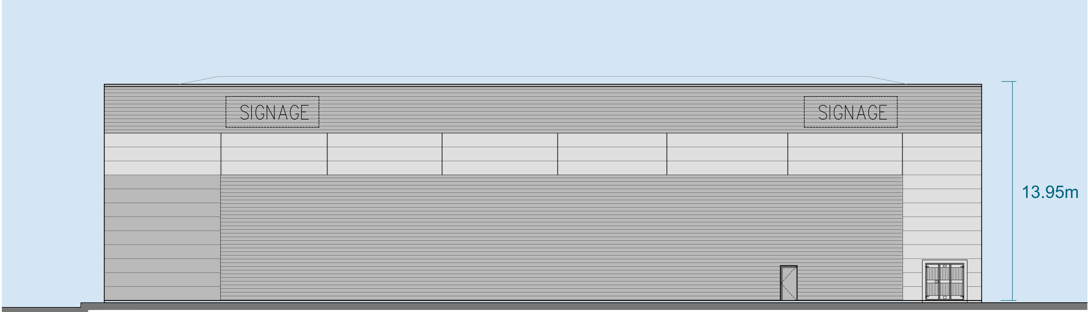
East Elevation
